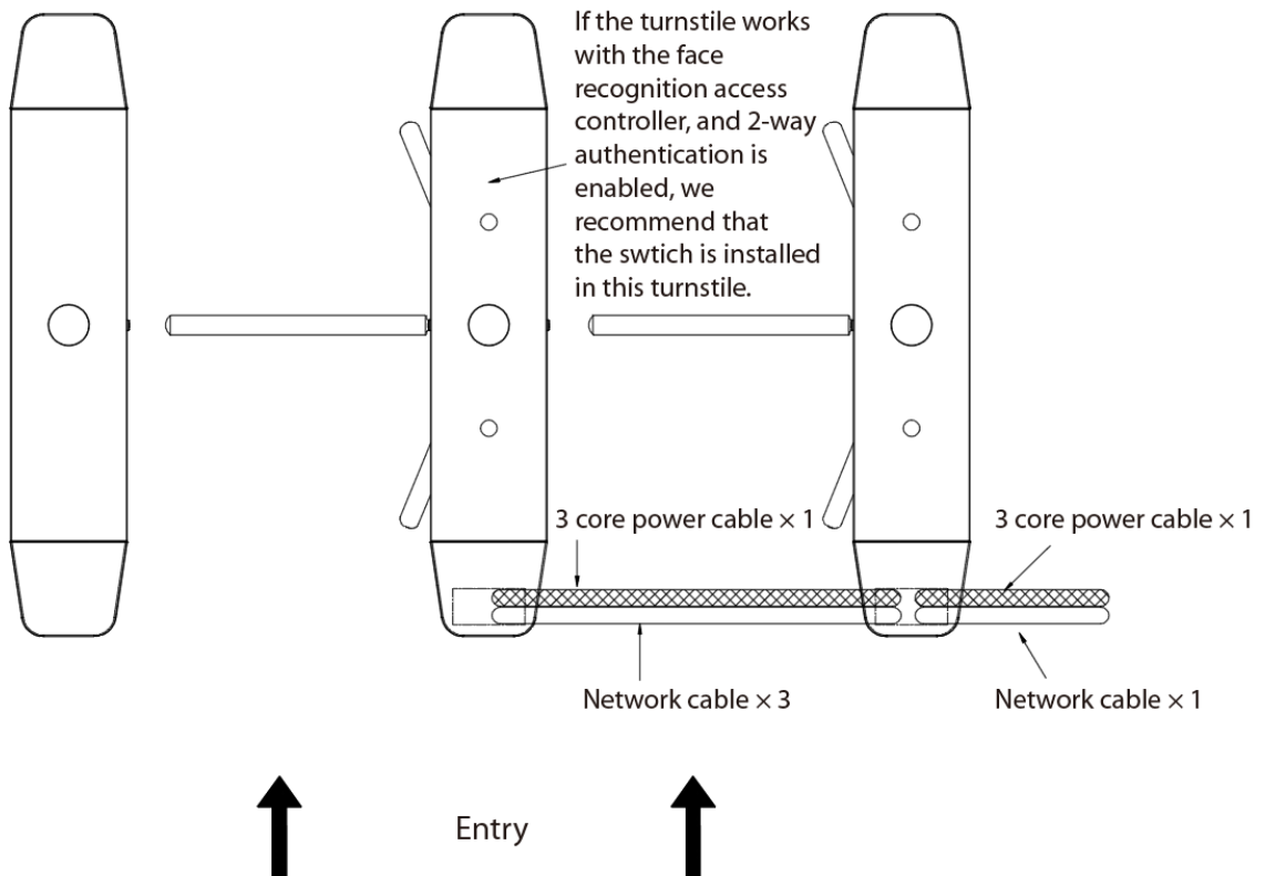
Figure 2-5 Wiring diagram
