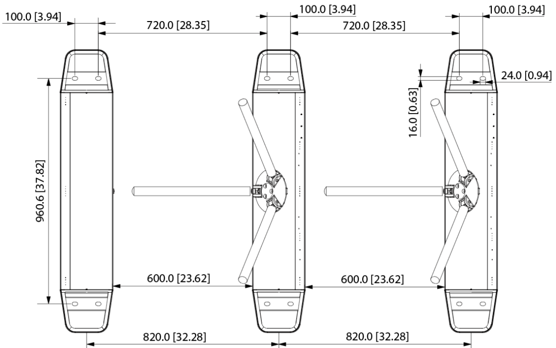
Figure 2-2 Hole drilling diagram (mm [inch])
