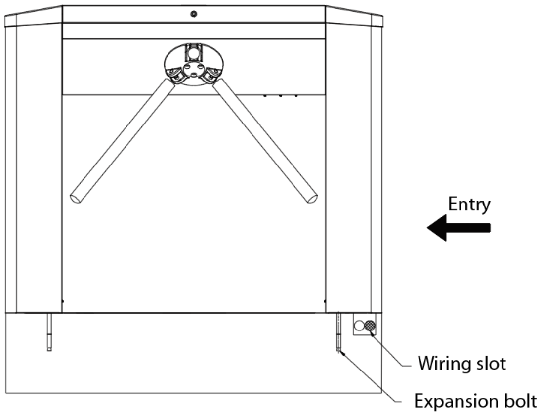
Figure 2-4 Wiring slot
