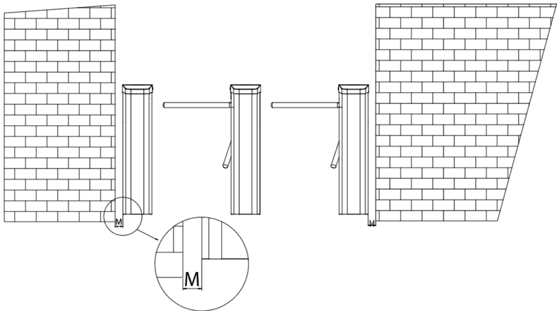
Figure 2-1 Spacing requirements
