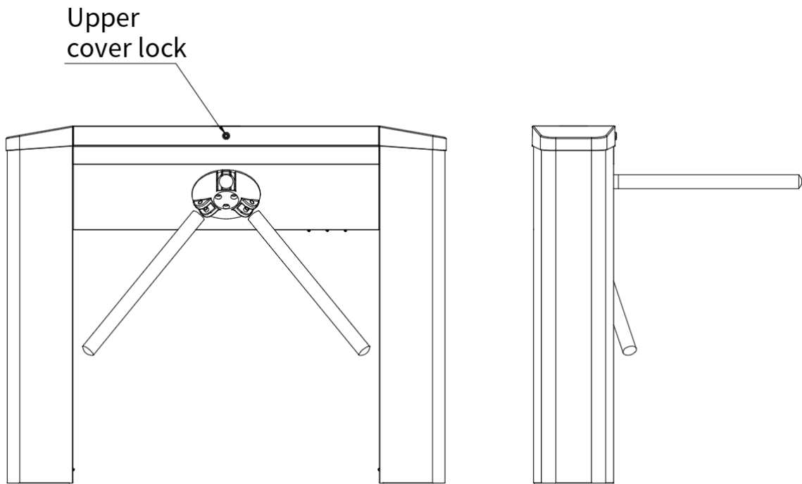
Figure 2-3 Turnstile doors
