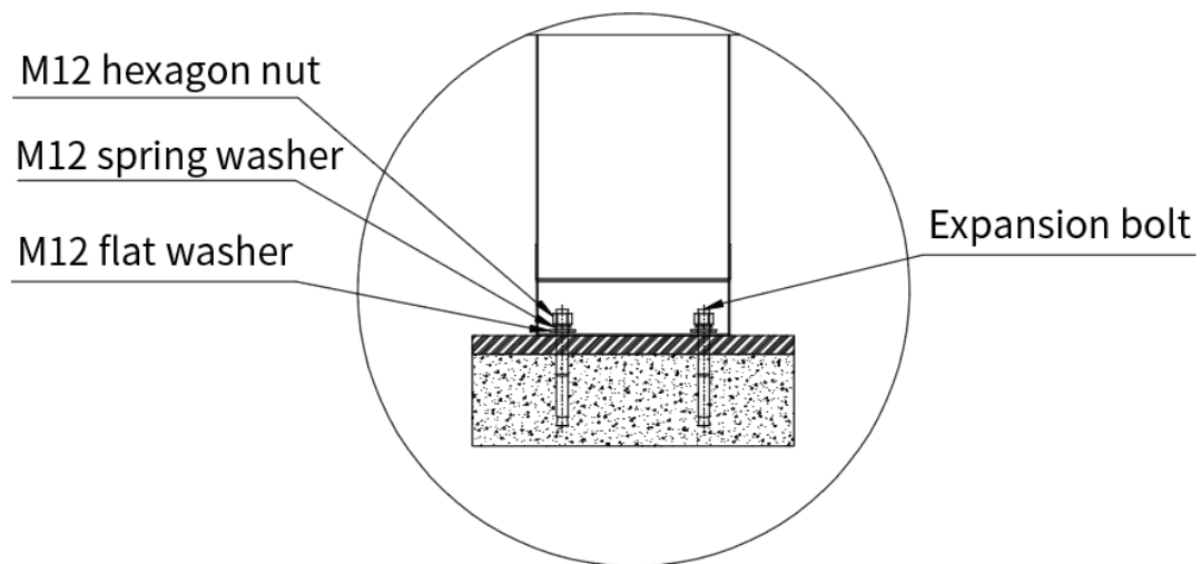
Figure 2-6 Secure turnstiles
