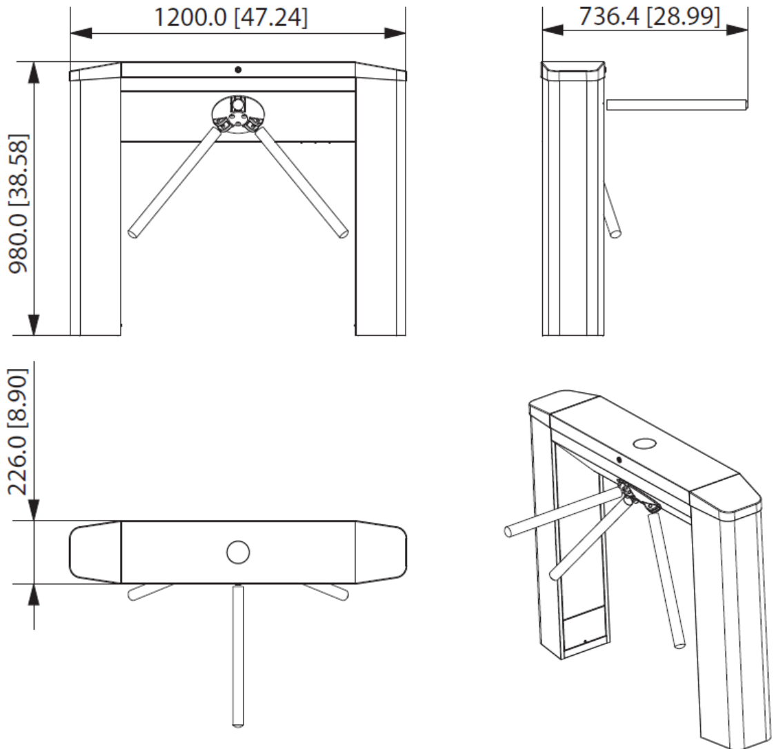
Figure 1-1 Dimensions (unit: mm [inch])
